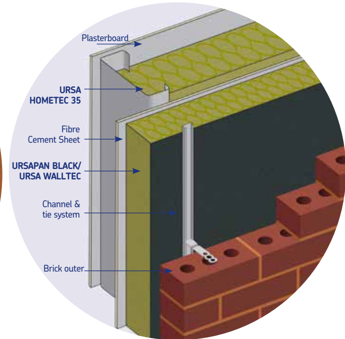
Figure 6 – Rainscreen Cladding with Brick Outer Leaf
