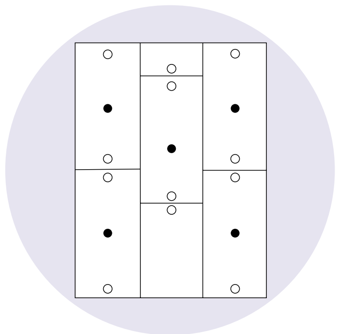
Figure 2 – Fixing Pattern
